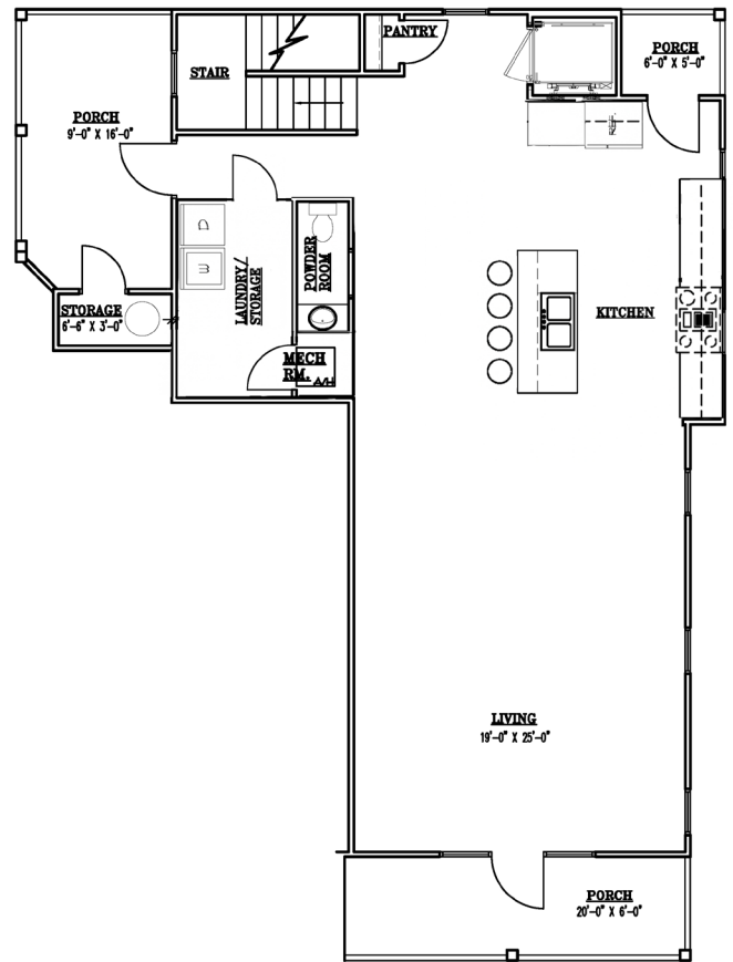
2nd floor
